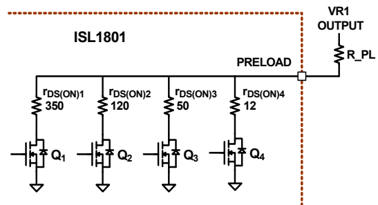
FIGURE 22. PRELOAD SWITCHES
