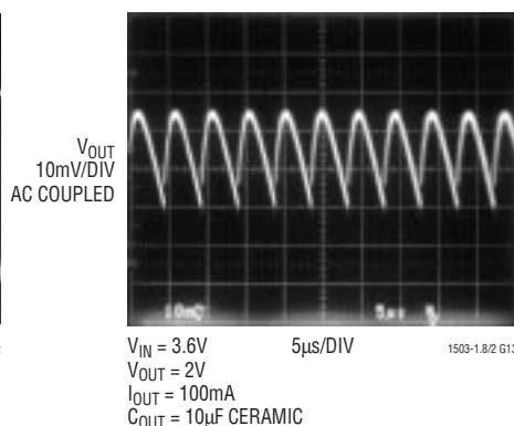
Output Ripple, C_{OUT} = 10\mu F
