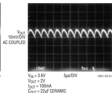
Output Ripple, C_{OUT} = 22\mu F
