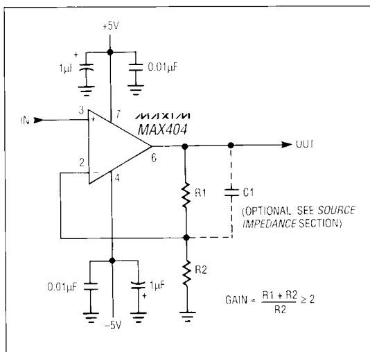
Figure 1. Noninverting Amplifier
