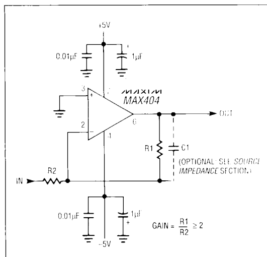
Figure 3. Inverting Amplifier
