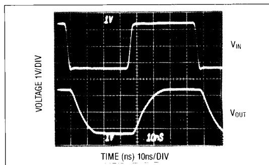
Figure 2. Noninverting Pulse Response
