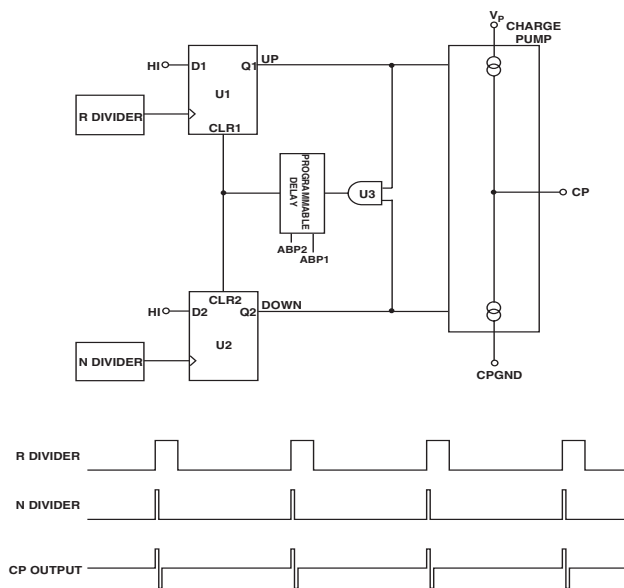
Figure 5. PFD Simplified Schematic and Timing (In Lock)
