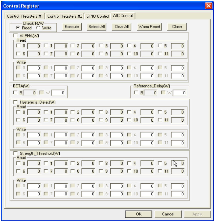
Figure 9: A Typical Parameter Window of Tuning System
