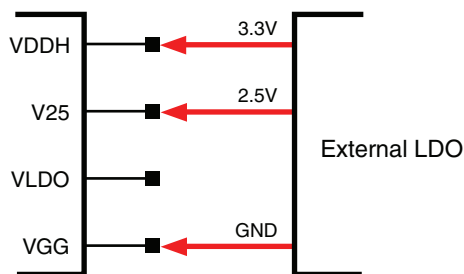
Case C. VDDH: External 3.3V VLDO: External 2.5V (Internal LDO Off: Register Control)
