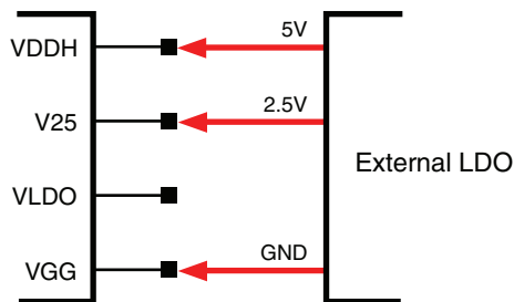
Case A. VDDH: External 5V VLDO: External 2.5V (Internal LDO Off: Register Control)
