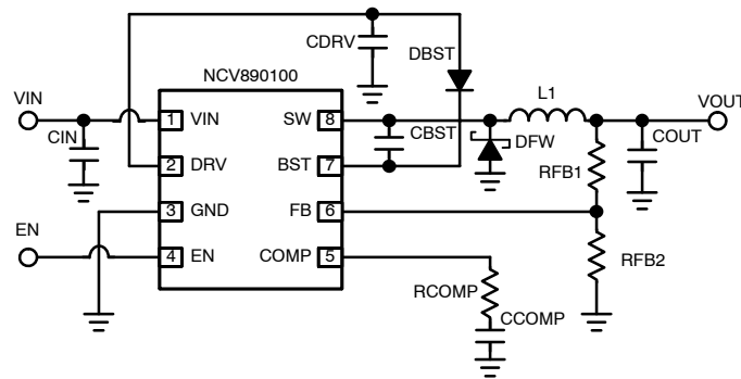
Figure 1. Typical Application
