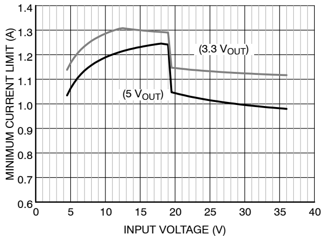
Figure 26. NCV890100 Load Current Capability with 4.7 \mu H Inductor
