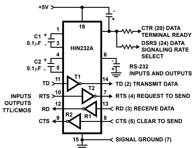
FIGURE 7. SIMPLE DUPLEX RS-232 PORT WITH CTS/RTS HANDSHAKING
