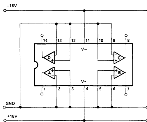
Burn-In Circuit
