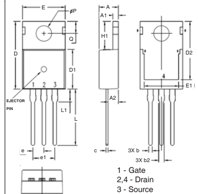
TO-220 Outline
