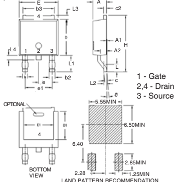
TO-252 AA Outline
