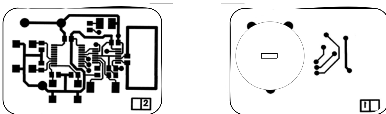
Figure 13. Two-Button Keyfob Board Layout
