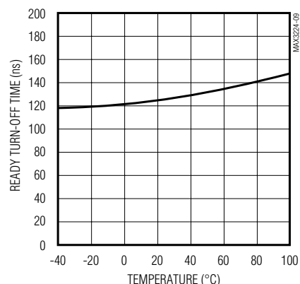
MAX3224–MAX3227 READY TURN-OFF TIME vs. TEMPERATURE
