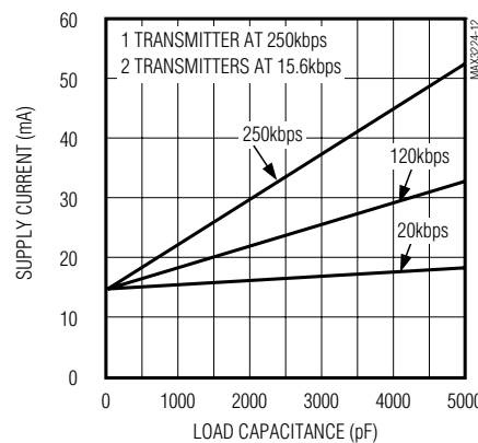
MAX3244 OPERATING SUPPLY CURRENT vs. LOAD CAPACITANCE
