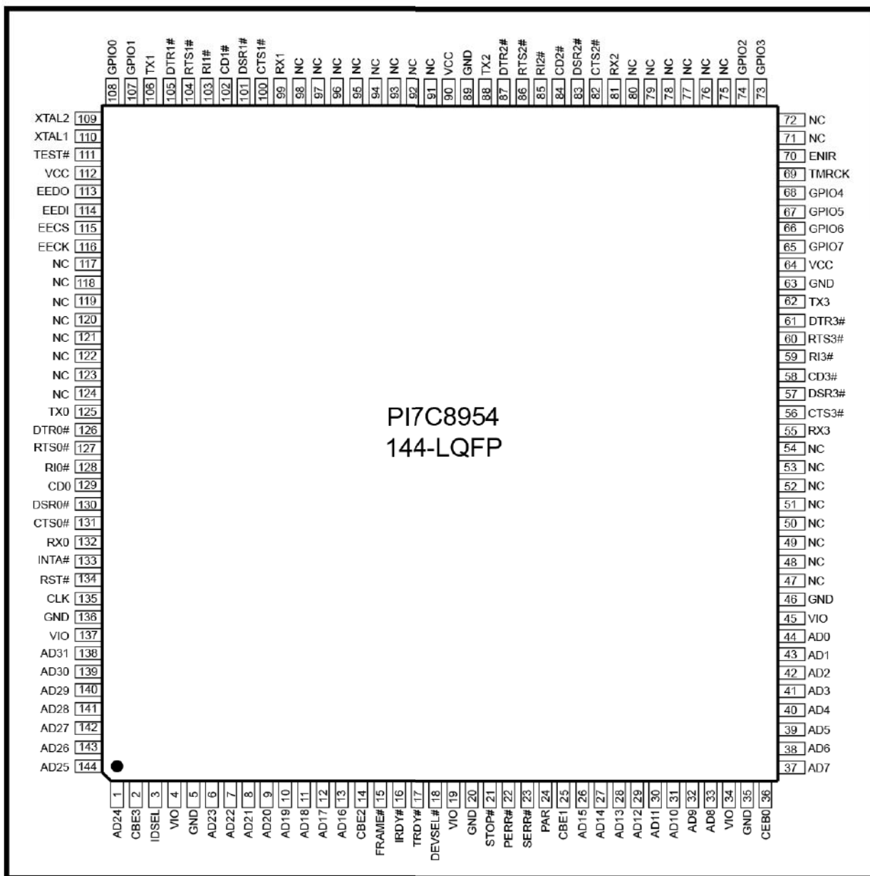
Figure 3-2 Pin Out
