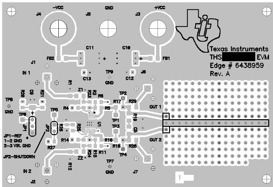
Figure 5–1. Top Layer 1 of THS6043EVM
