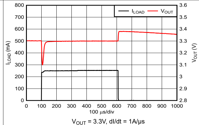
Figure 5-42. Load Transient Response (New Chip)
