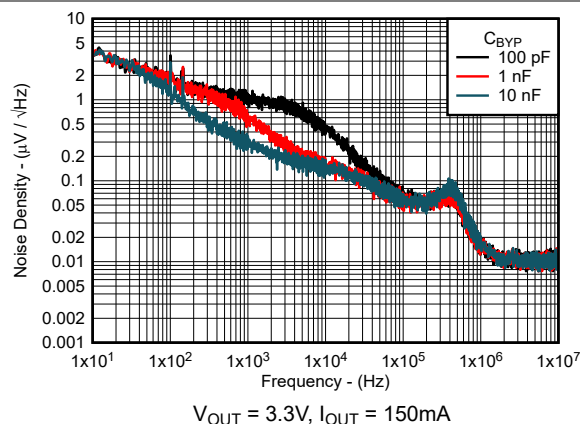
Figure 5-26. Output Noise Density vs Frequency (New Chip)
