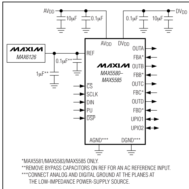
Figure 10. Bypassing Power Supplies \text{AV}_{\text{DD}} , \text{DV}_{\text{DD}} , and REF
