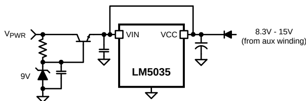
Figure 17. Start-Up Regulator for V_{PWR} > 100\text{ V}
