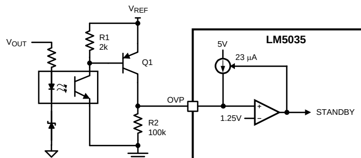
Figure 24. Latched Load Overvoltage Protection
