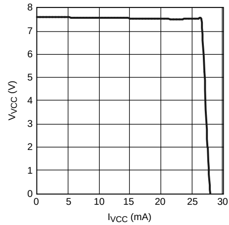
Figure 2. V VCC vs I VCC
