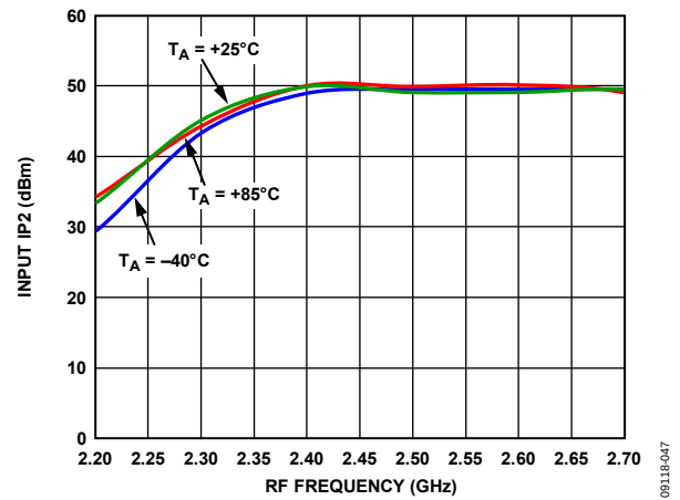
Figure 48. Input IP2 vs. RF Frequency at 3.3 V
