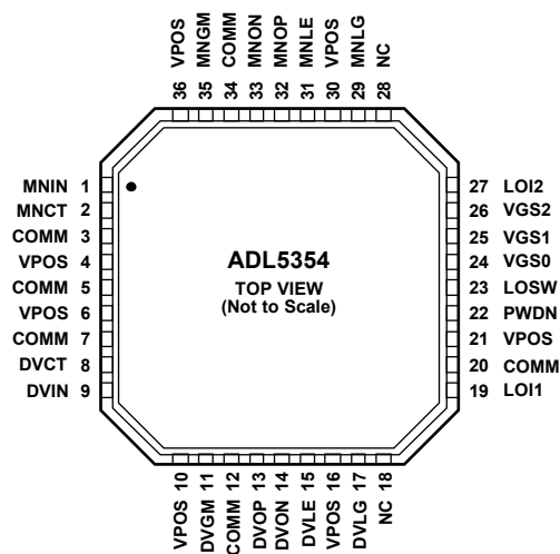
Figure 2. Pin Configuration
