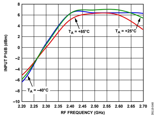
Figure 49. Input P1dB vs. RF Frequency at 3.3 V
