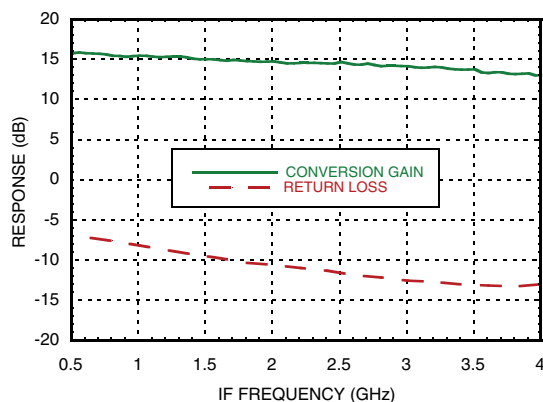
IF Bandwidth [1]
