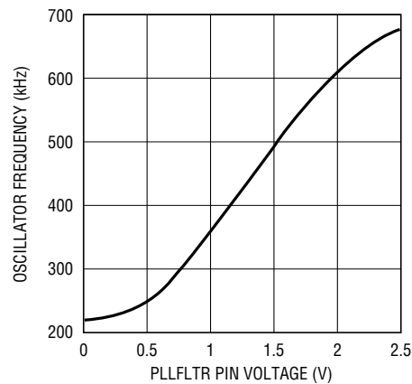
Oscillator Frequency vs V_{PLLFLTR}
