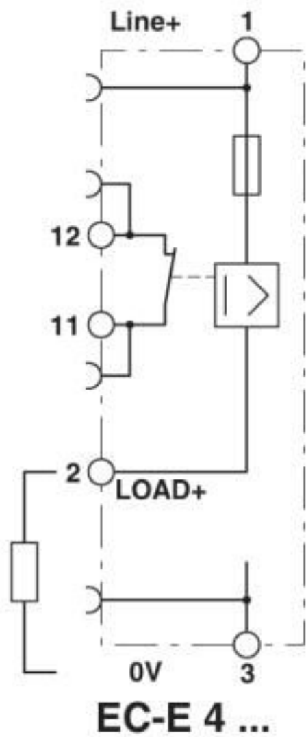
Circuit diagram
