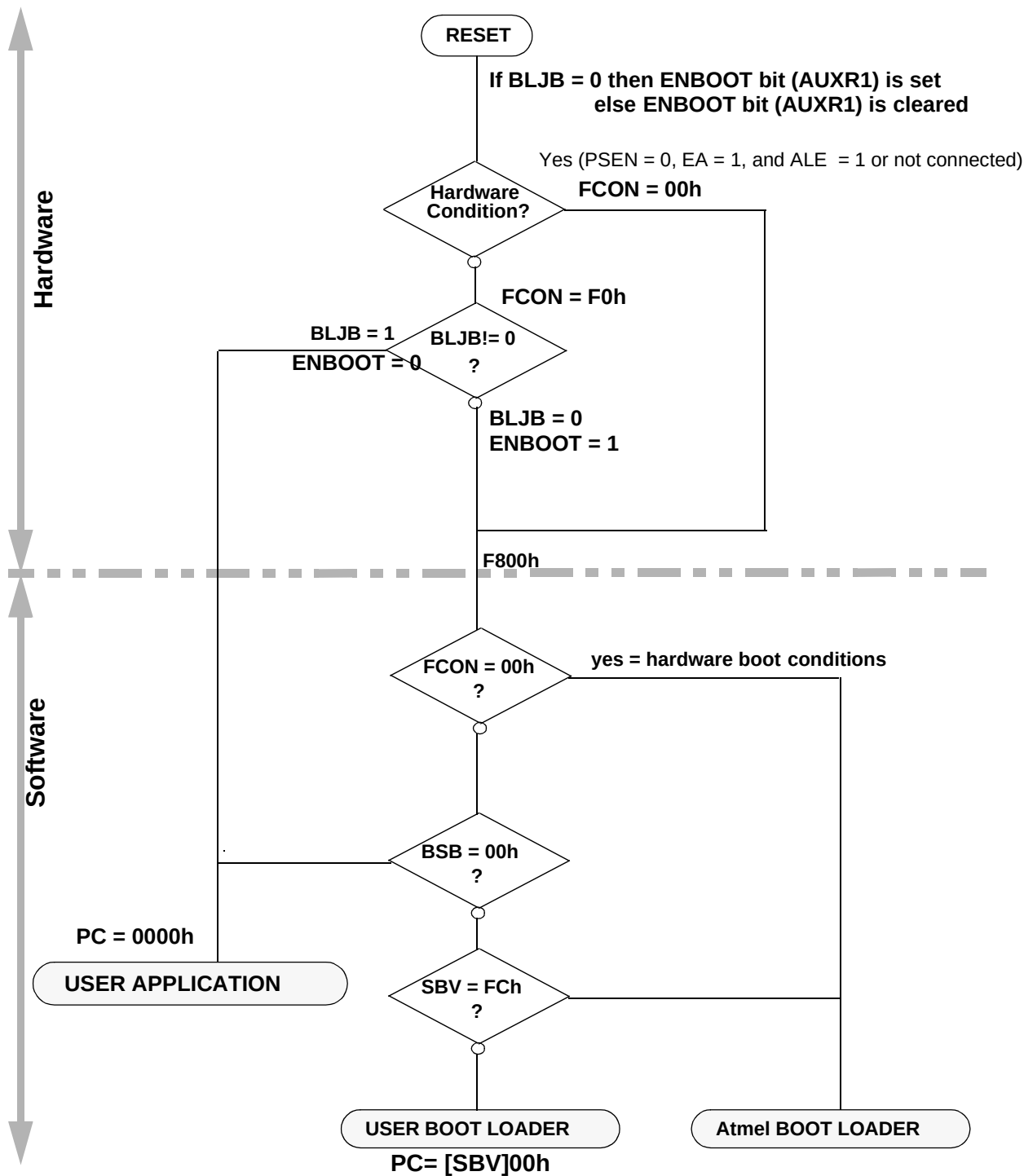
Figure 46. Bootloader process
