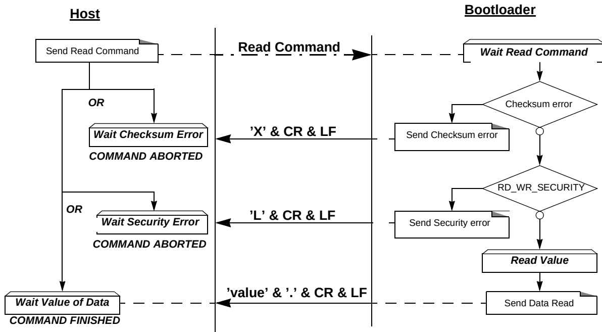
Figure 52. Read Flow
