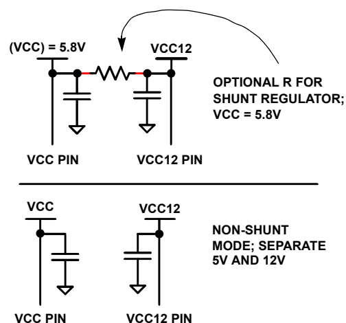
FIGURE 11. SHUNT REGULATOR AND DECOUPLING CAPACITORS FOR VCC AND VCC12 PINS
