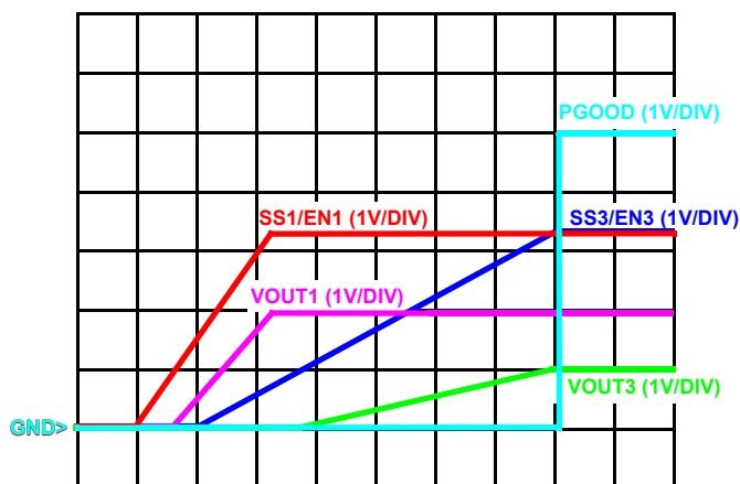
FIGURE 10. PGOOD OUTPUT
