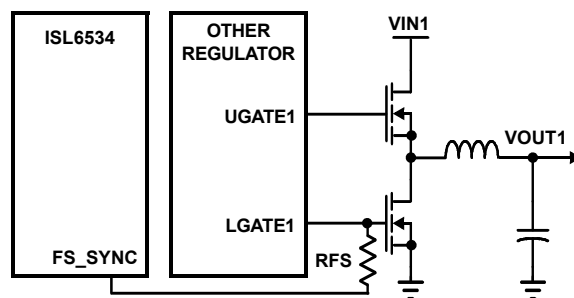
FIGURE 13. CONNECTION OF FS_SYNC TO THE LGATE OF ANOTHER SWITCHING REGULATOR
