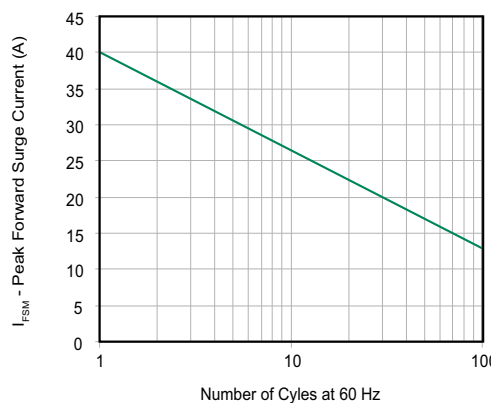
Figure 7 - Maximum Non-Repetitive Forward Surge Current Uni-Directional Only
