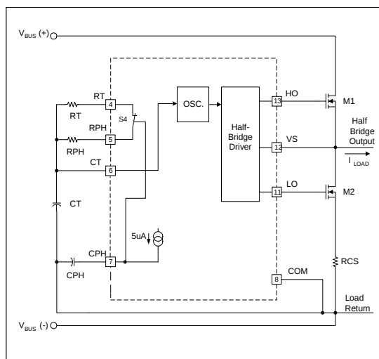
Figure 3, Preheat circuitry
