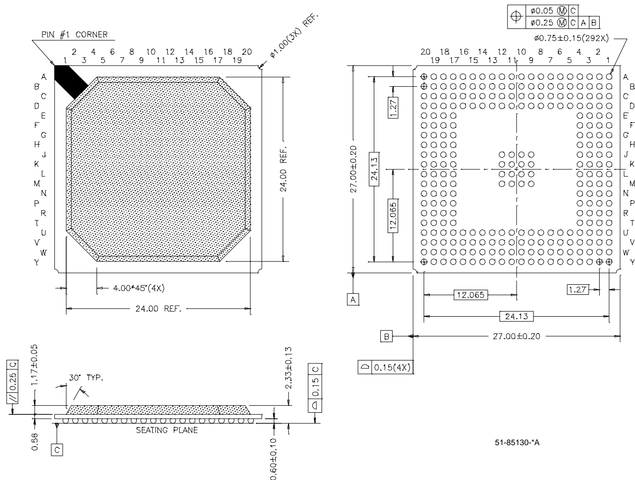
Figure 20-1. Package
