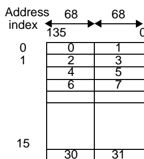
Figure 7-1. Comparand-Register Selection During Search and Learn Instructions
