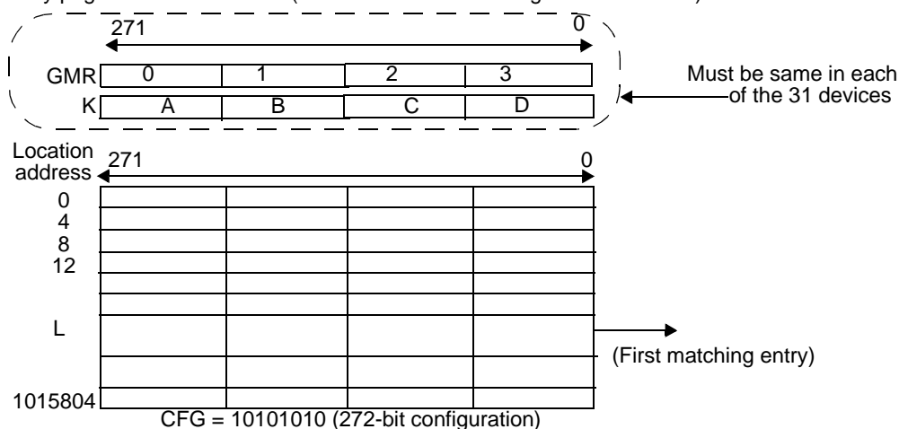
Figure 10-70. x272 Table with 31 Devices
