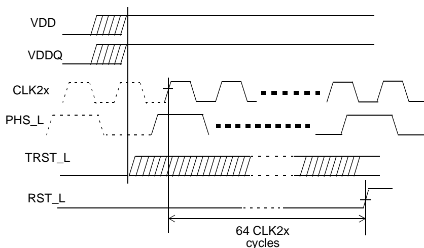
Figure 13-1. Power-up Sequence
