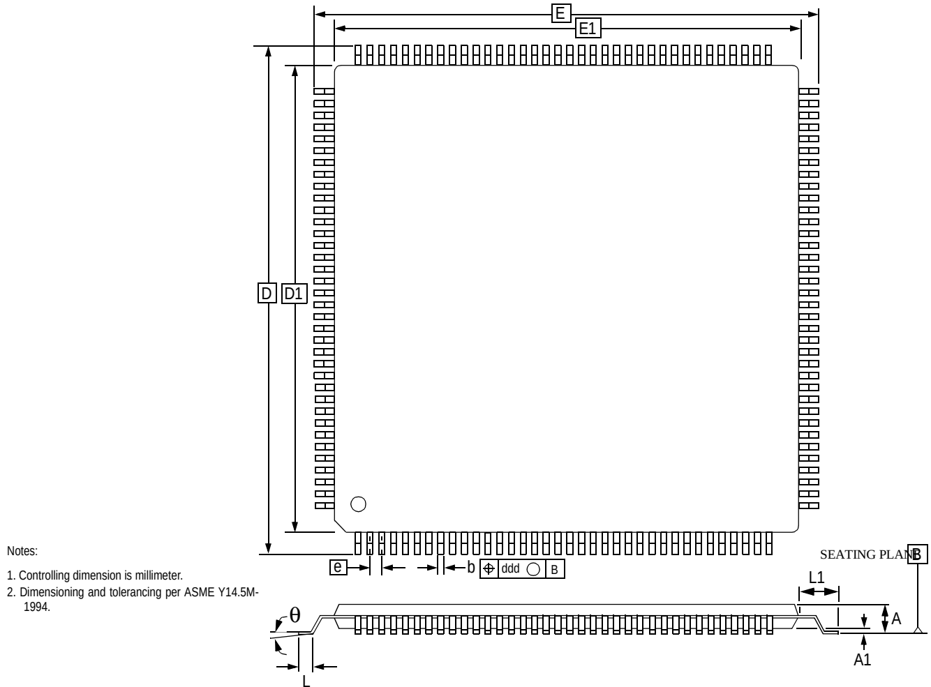
Figure 24. 144-Pin LQFP Package Drawing
