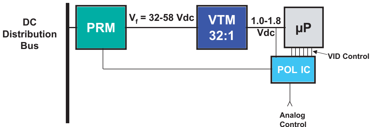
Figure 31—PRM and VTM, Closed loop with VID Controller
