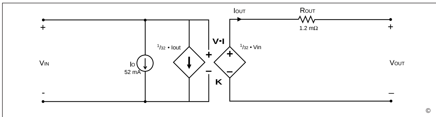
Figure 27 —This model characterizes the DC operation of the V•I Chip VTM, including the converter transfer function and its losses. The model enables estimates or simulations of output voltage as a function of input voltage and output load, as well as total converter power dissipation or heat generation.
