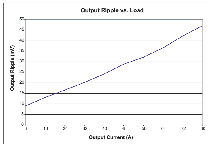
Figure 10 — Output voltage ripple vs. output current at nominal line with no POL bypass capacitance.
