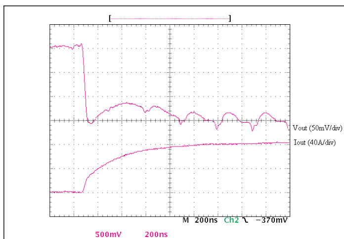
Figure 11 — 0-80A step load change with 100 \mu F input capacitance and no output capacitance.
