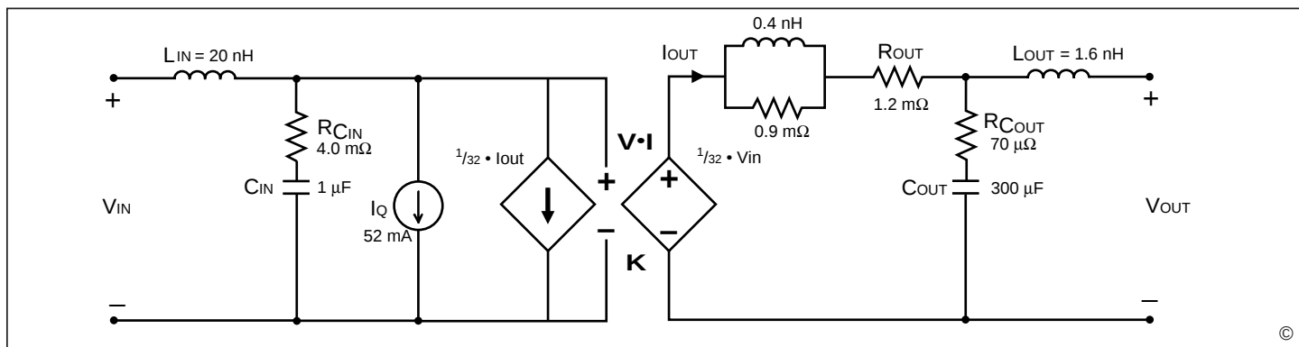
Figure 28 —This model characterizes the AC operation of the V•I Chip VTM including response to output load or input voltage transients or steady state modulations. The model enables estimates or simulations of input and output voltages under transient conditions, including response to a stepped load with or without external filtering elements.
