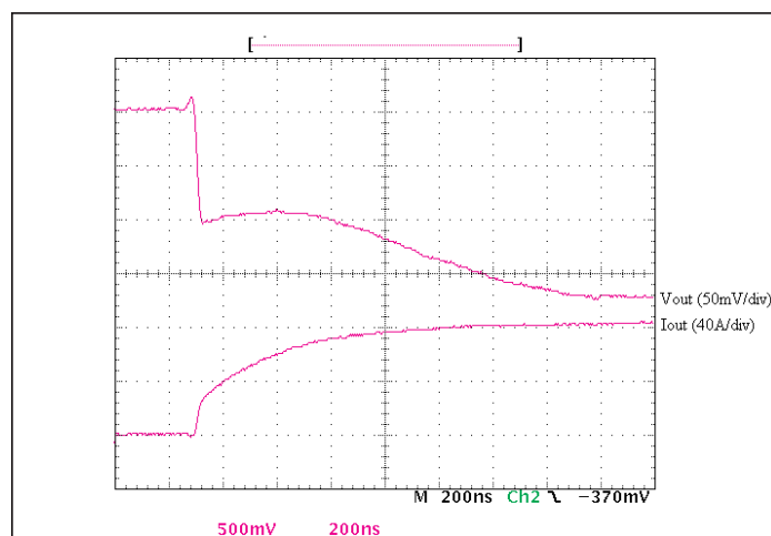
Figure 12 — 0-80A step load change with 100 \mu F input capacitance and 100 \mu F output capacitance.
