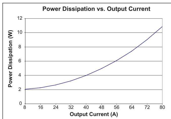
Figure 6—Power dissipation as a function of output current at 1.5V V OUT
