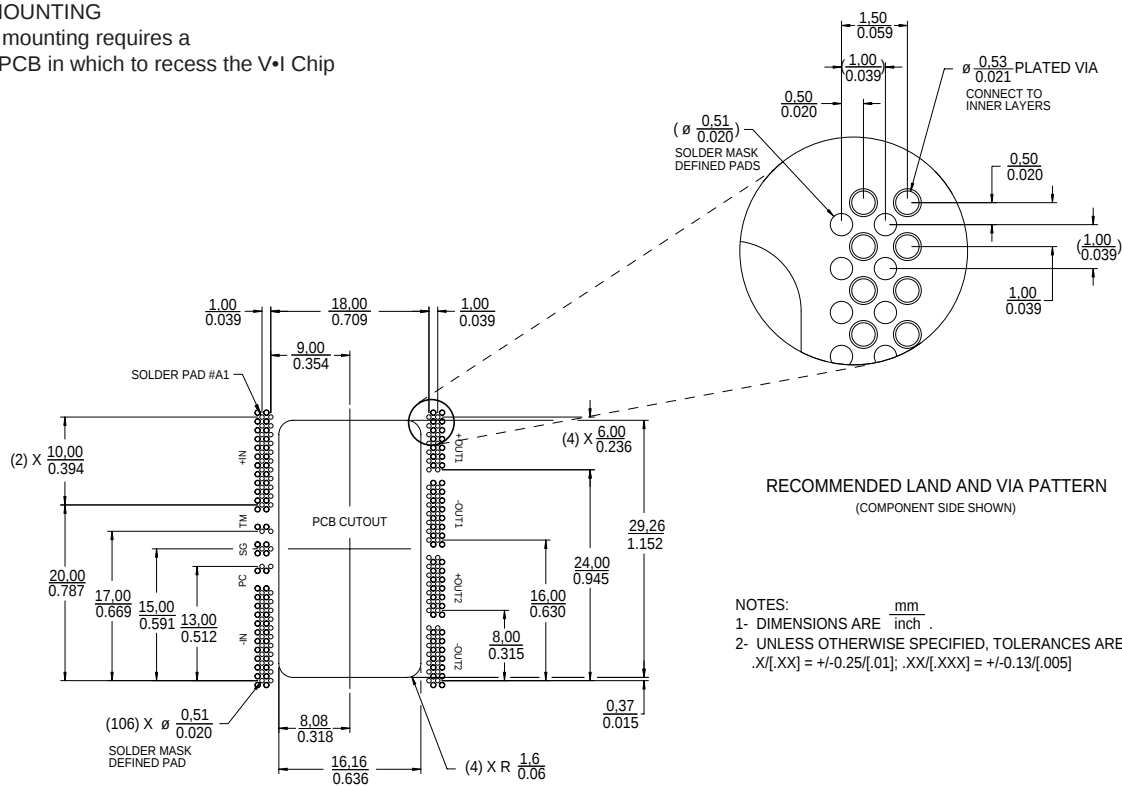
Figure 17—VTM BGA PCB land/VIA layout information; In-board mounting
