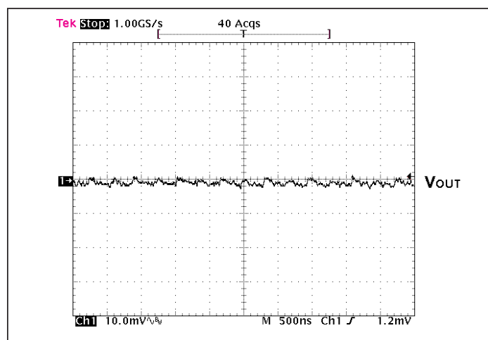
Figure 8 —Output voltage ripple at full load and nominal V_{IN} with 200 \mu F ceramic external bypass capacitance.
