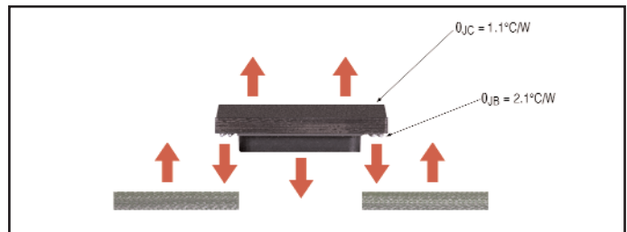
Figure 25 —Thermal resistance
