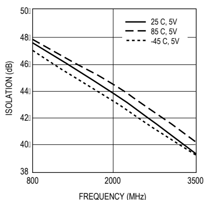
Figure 17. Isolation vs. Frequency. □ ( P_{in} = -10 dBm, V_d = 5 V)
