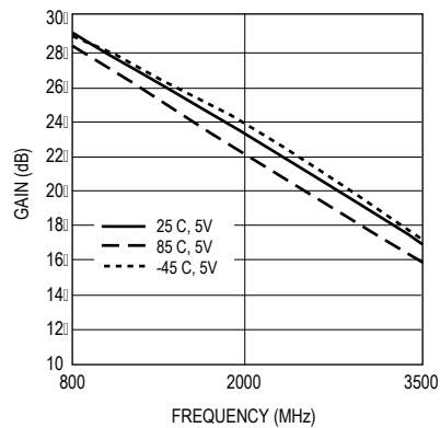
Figure 15. Gain vs. Frequency. □ ( P_{in} = -10 dBm, V_d = 5 V)
