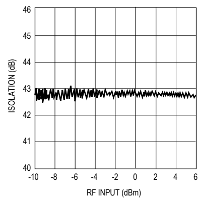
Figure 8. Isolation vs P_{in} , V_d = 3V .
