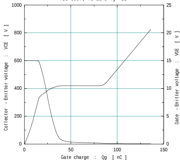
Dynamic Gate charge (typ.) Vcc=600V, Ic=15A, Tj= 25
