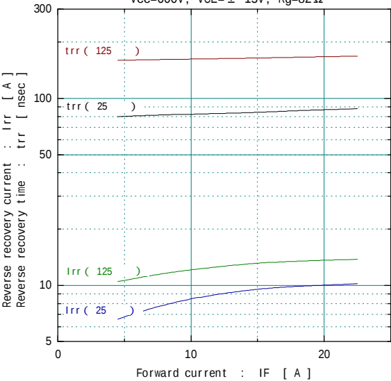
Reverse recovery characteristics (typ.) Vcc=600V, VGE=± 15V, Rg=82Ω
