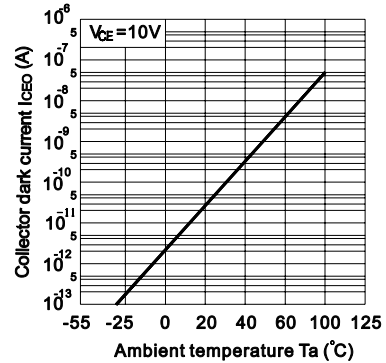
Fig.8 Collector Dark Current vs. Ambient Temperature
