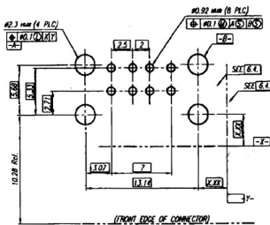
FIGURE A: PCB FOOTPRINT FOR RECEPTACLE (THROUGH-HOLE)
