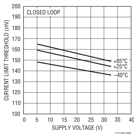
Current Limit Threshold
