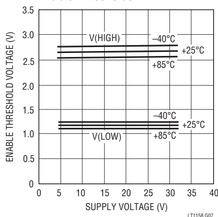
Enable Thresholds
