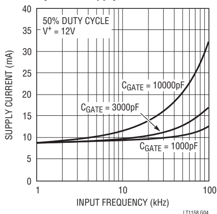
Dynamic Supply Current
