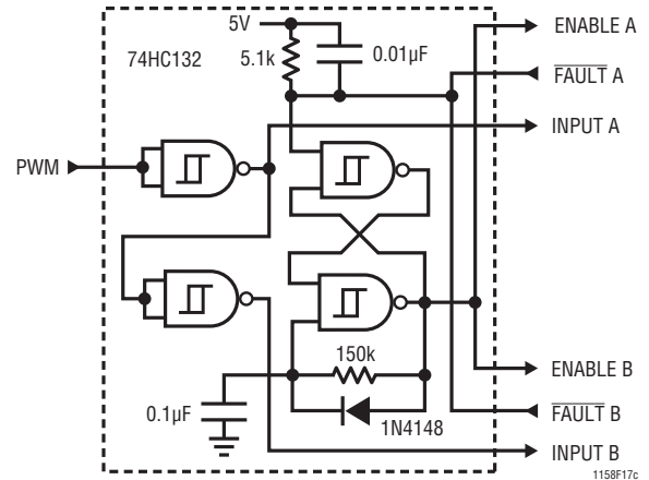
Figure 17. 10A Full Bridge Motor Control
