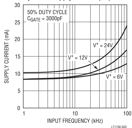
Dynamic Supply Current ( V^+ )
