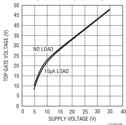
Charge Pump Output Voltage
