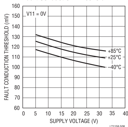
Fault Conduction Threshold
