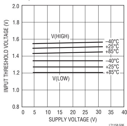
Input Thresholds
