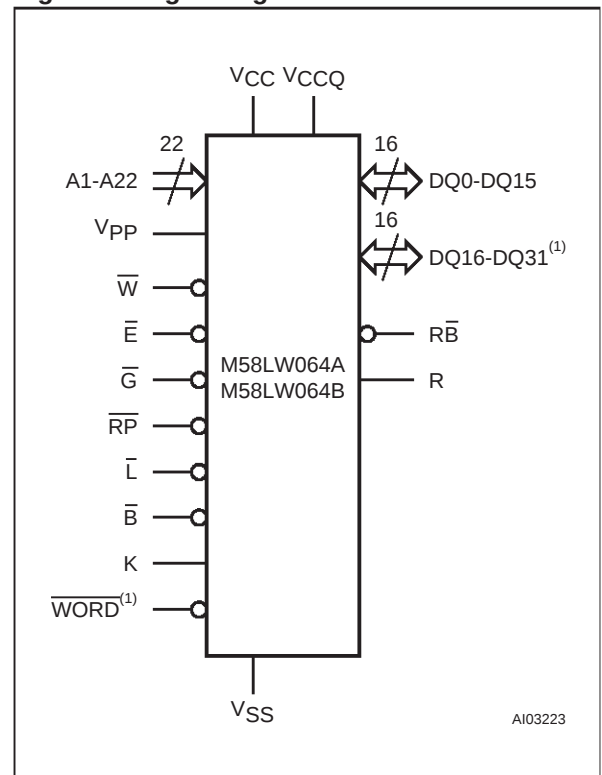
Figure 1. Logic Diagram
