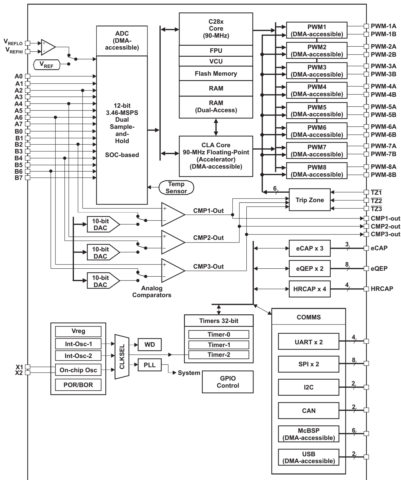
Figure 1-2. Peripheral Blocks
