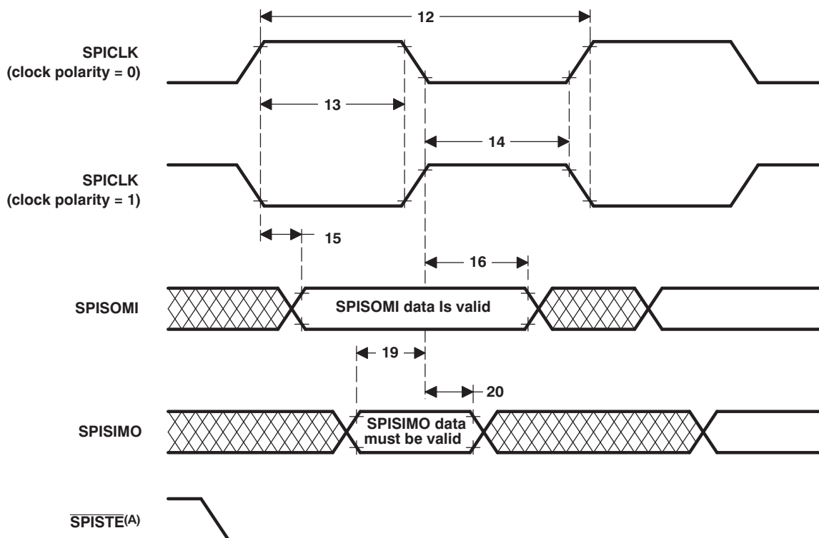
Figure 5-29. SPI Slave Mode External Timing (Clock Phase = 0)
