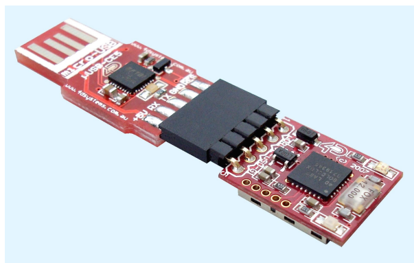
uDRIVE with uUSB-CE5 Interface
