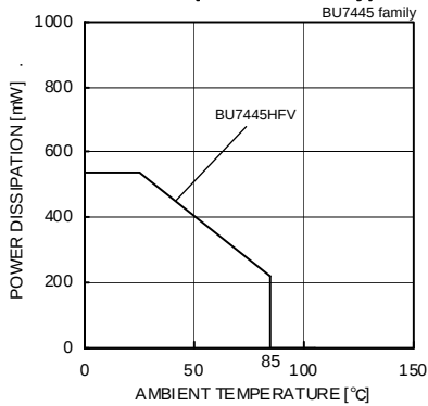
Fig.162 Derating curve
