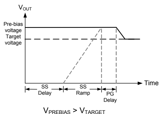
Figure 20. Output Response to Pre-Bias Voltages
