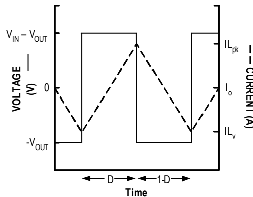
Figure 7. Inductor Waveform
