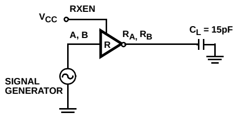
FIGURE 7A. TEST CIRCUIT
