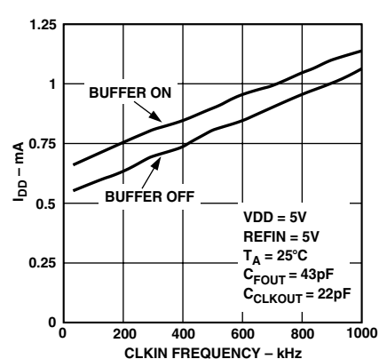
TPC 6. IDD vs. CLKIN (Buffered and Unbuffered)
