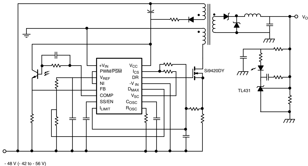
Figure 2. Si9118 15 W Forward Converter Schematic
