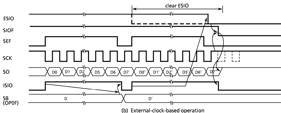
Figure 3-29. Transmit Mode
