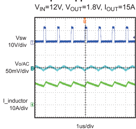
Output Ripple
