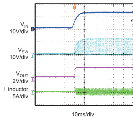
Power up
