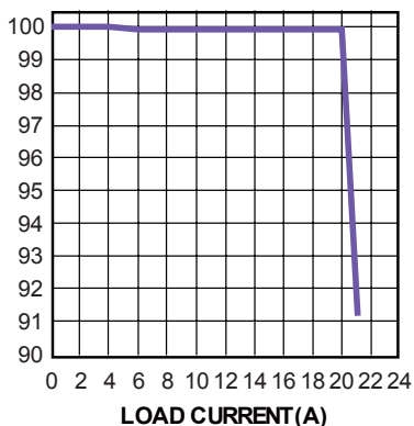
Load Regulation
