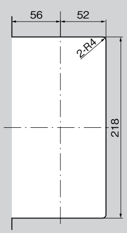
パネル穴明け寸法 (右開き用) Panel drilling dimensions (for right-hand use)
