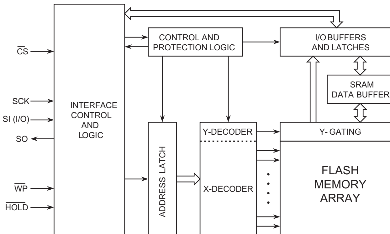
Figure 3-1. Block Diagram
