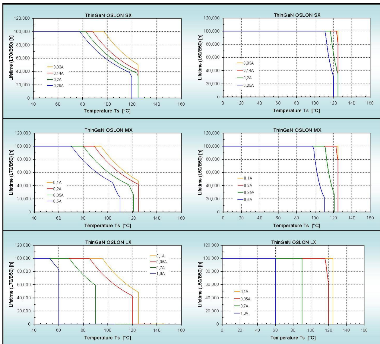
Figure 5a: Lifetimes (*) of the OSOLON types (SX, MX, LX) with ThinGaN technology with respect to T_S
