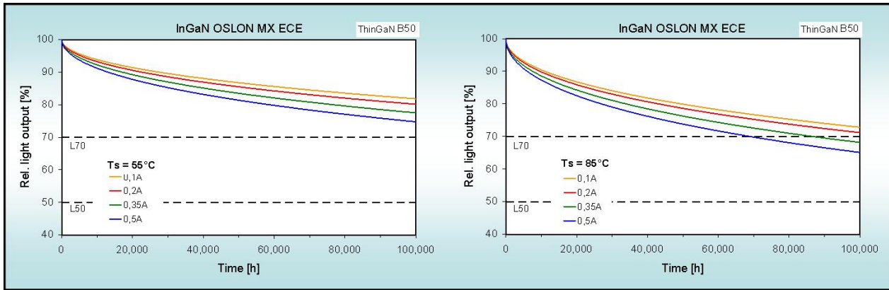
Figure 6e: Degradation characteristics (*) of the OSLON MX ECE (LxW CN7N) for T_s=55^\circ\text{C} & T_s= 85^\circ\text{C} (grouping current I_F = 0,35\text{A} )
