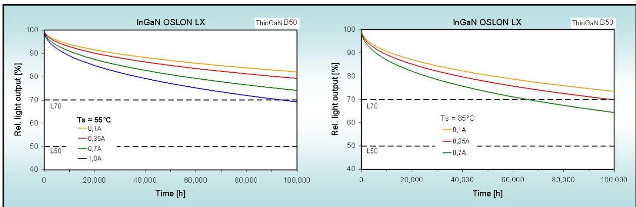
Figure 6c: Degradation characteristics (*) of the OSLOM LX (LxW CNAP) for T_s=55^\circ\text{C} & T_s=85^\circ\text{C} (grouping current I_F = 0,35\text{A} )
