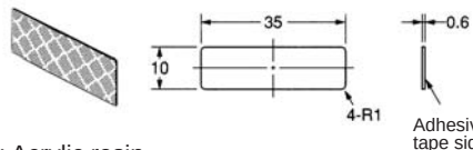
E39-RS1 Retroreflector
