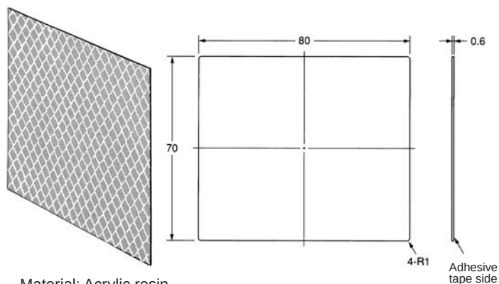
E39-RS3 Retroreflector
