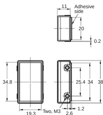
E39-RS1 Retroreflector
