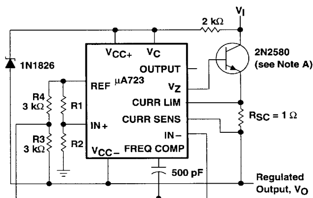
Figure 5. Positive-Voltage Regulator (External P-N-P Pass Transistor)
