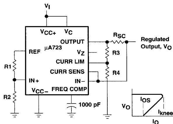
Figure 6. Foldback Current Limiting
