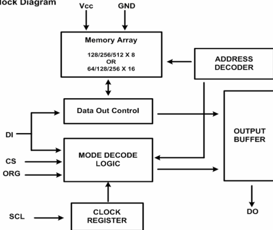
Block Diagram
