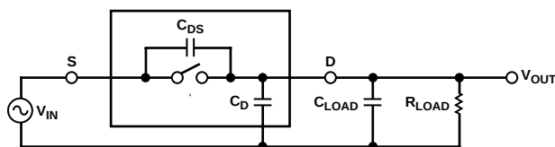
Figure 8. Off Isolation Is Affected by External Load Resistance and Capacitance
