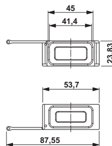
Protective cover for D-SUB
